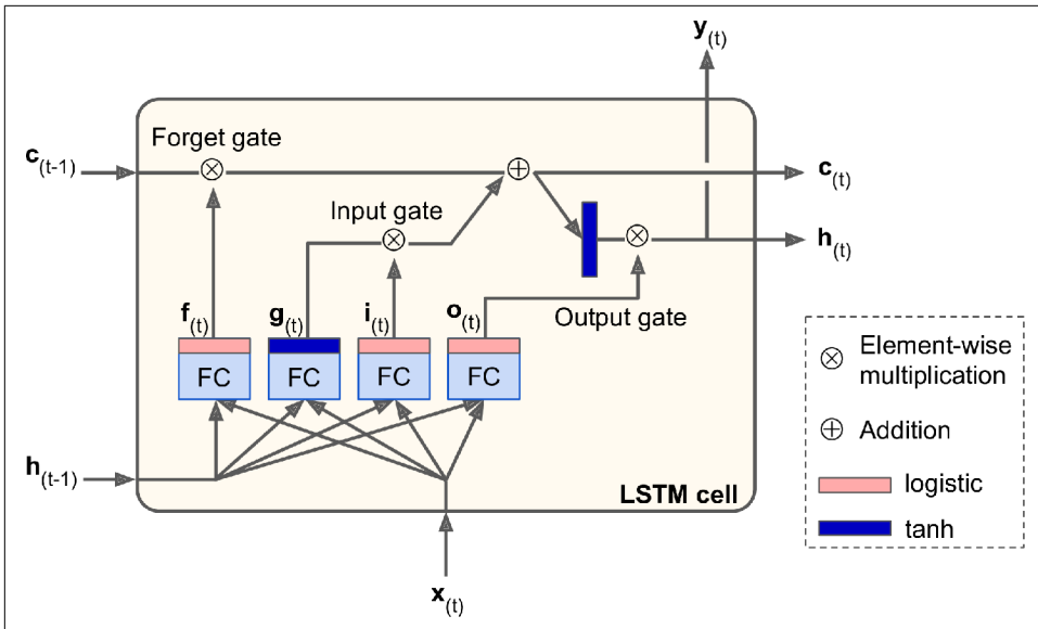
Figure 15-9. LSTM cell
