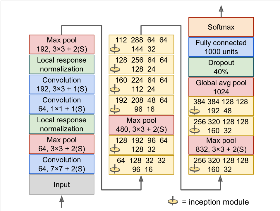
Figure 14-14. GoogLeNet architecture
