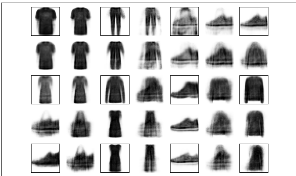
Figure 17-14. Semantic interpolation
