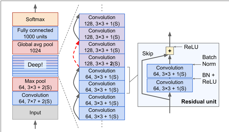
Figure 14-17. ResNet architecture
