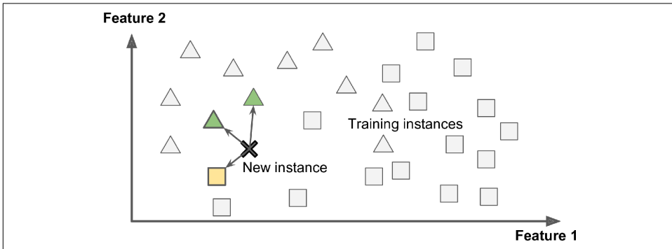
Figure 1-15. Instance-based learning
