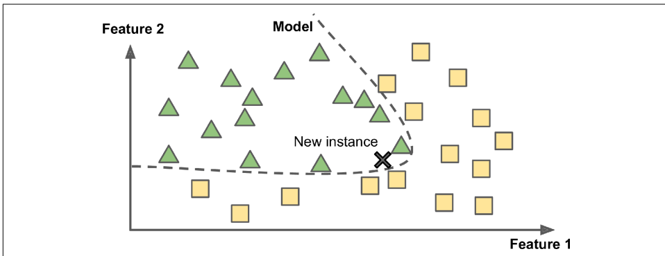
Figure 1-16. Model-based learning
